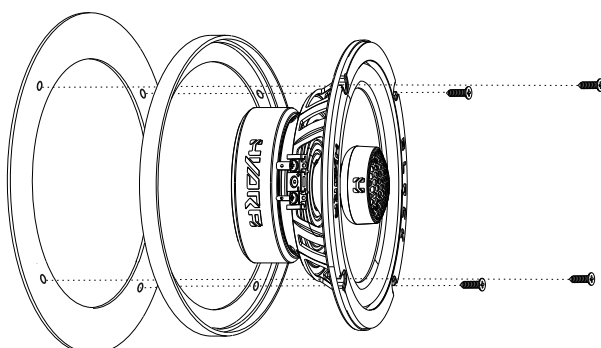
Installation of the coaxial speaker with use of spacers
