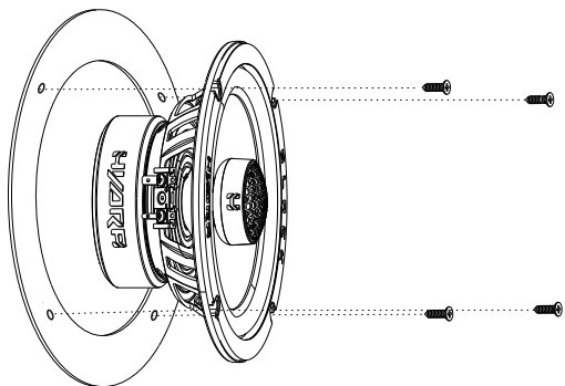
Installation of the coaxial speaker
